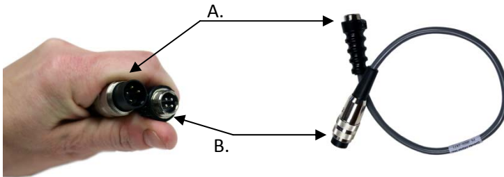
A. 4-pin Male OverView Connector B. 4-pin Male Lumberg Circular Din Connector
