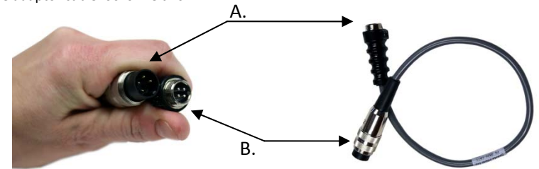
A. 4-pin Male OverView Connector B. 4-pin Male Lumberg Circular Din Connector
