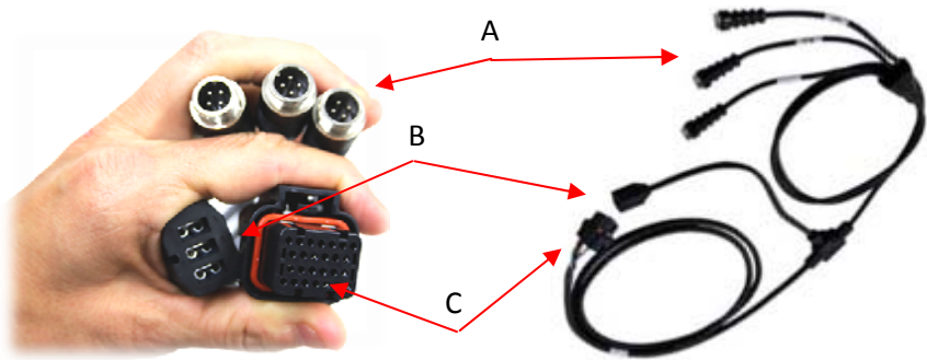
A. John Deere Power Input Plug B. 26-pin Tyco Connector C. 4-pin Male OverView Connectors (Qty 3)
