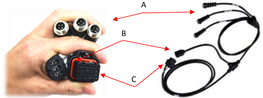
A. John Deere Power Input Plug B. 26-pin Tyco Connector C. 4-pin Male OverView Connectors (Qty 3)
