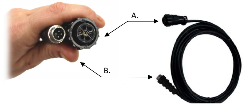
A. Round AMP Connector B. 4-pin Male OverView Connector
